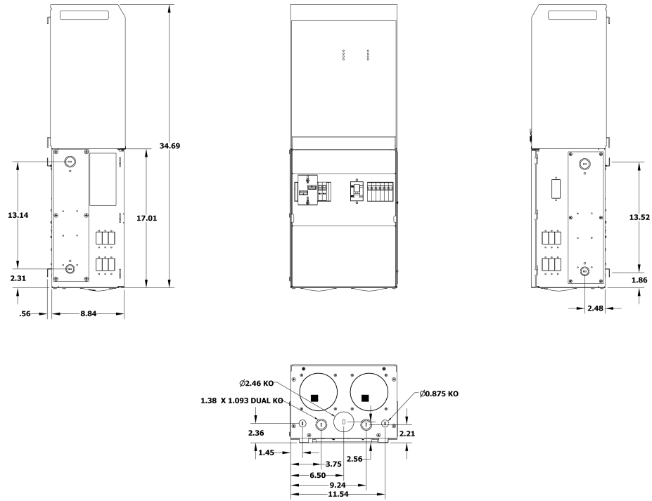
Figure 3 - 5k VE Panel Dimensions
