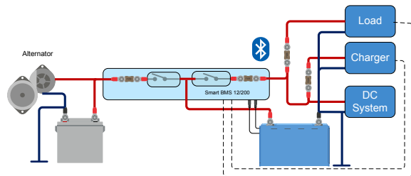
The Smart BMS 12/200 will disconnect loads and chargers or turn loads and chargers off via "load disconnect" and "charge disconnect" signals. It also controls and limits the alternator.
