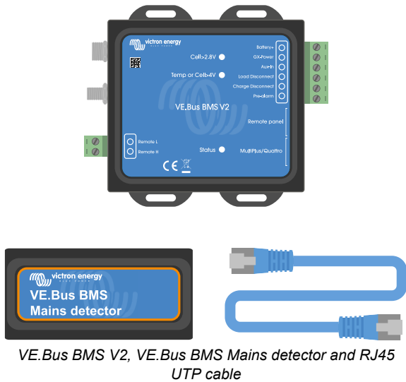
The VE.Bus BMS V2 will turn loads and chargers off via “load disconnect”, and “charge disconnect” and controls the inverter/charger
