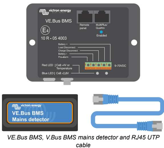
The VE.Bus BMS will turn loads and chargers off via “load disconnect”, and “charge disconnect” and controls the inverter/charger
