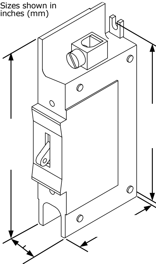
Figure 1, Physical Dimensions
